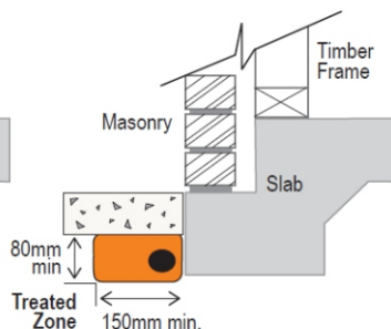
Pipe clipped low on footing
